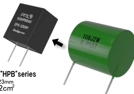
FilmCAP "PCK" series 26 x 25.5 x 27.5mm 18.23cm 3
